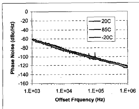
Fig 6. Bipolar Phase Noise vs. Temperature
