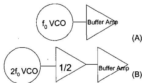
Fig.1 Block diagram of two VCO system configurations
